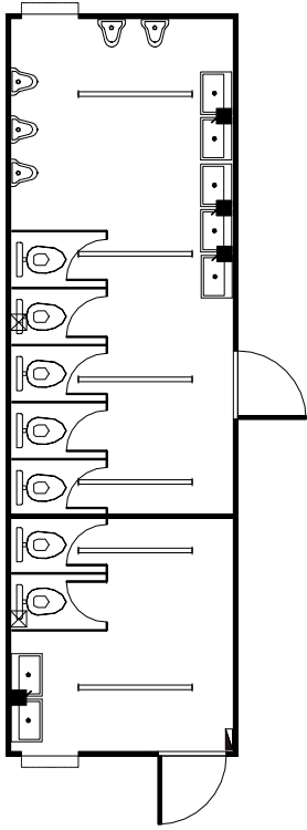
5+2 layout
